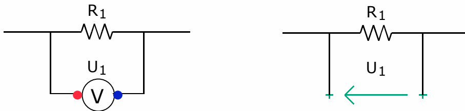
U1 is the voltage measured by the voltmeter.
